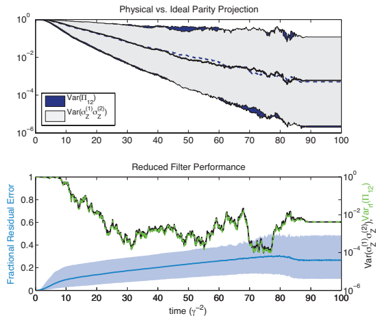
FIG. 3: Summary of 1000 Bell-state projection simulations. The top graph compares the statistics of the ideal and physical parity variance. The mean of the \text{Var}(\sigma_Z^{(1)} \sigma_Z^{(2)}) trajectories is shown as a solid, black line; grey shading indicates the one-standard deviation range of trajectories above and below the mean. The mean and standard deviation range of \text{Var}(\Pi_{12}) are shown by the dotted line and blue shading. The bottom graph highlights the performance of the reduced filter. Referenced to the right axis, a representative \text{Var}(\sigma_Z^{(1)} \sigma_Z^{(2)}) , \text{Var}_{r,f}(\Pi_{12}) trajectory pair are shown in solid black and dotted green, respectively. The blue-grey line and shading, referenced to the left axis, depicts the mean and standard deviation range of the fractional residual error over all trajectories.
