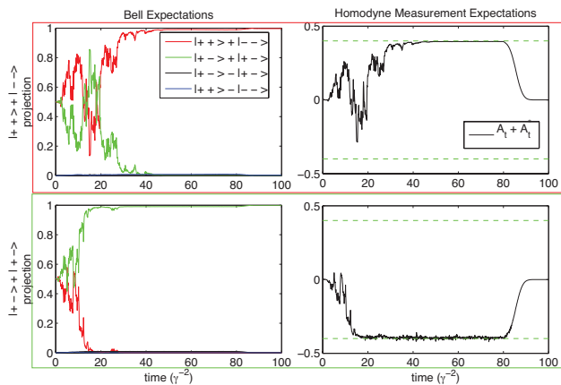
FIG. 2: Two independent simulations of atomic Bell-state preparation in a realistic system (see text). The top pair of graphs show a simulation in which the system happened to reduce to even parity; the bottom pair shows an odd-parity example.
