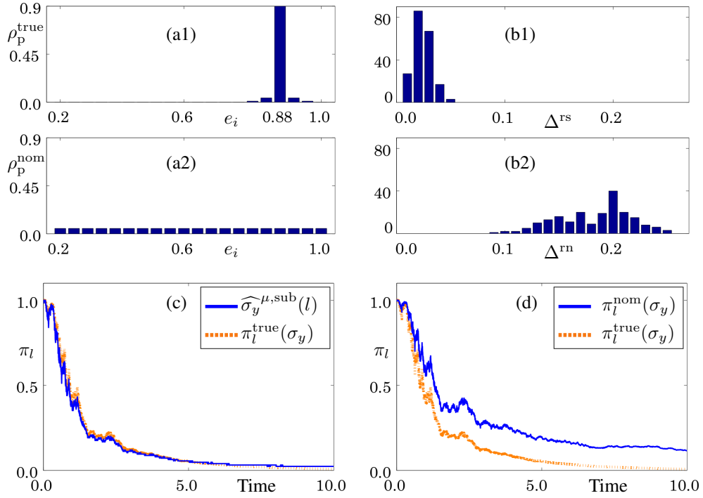
Fig. 3. For the spontaneous emission model of the atom, (a) the true and nominal parameter distributions, (b) the histogram of the averaged total estimation errors, (c) sample paths of the nominal risk-sensitive estimator (solid line) and the true risk-neutral one (thick dotted line), and (d) sample paths of the nominal risk-neutral estimator (solid line) and the true risk-neutral one (thick dotted line). For the figures (c) and (d), the notation ( \iota ) is omitted.
